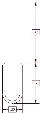
VIEW A-A SCALE 1/4"=1"
